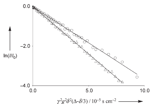
Figure 3. Stejskal–Tanner plot of 1-4BF 4 (○) and 2 (△) at 297 K in [\text{D}_1]\text{chloroform} .
