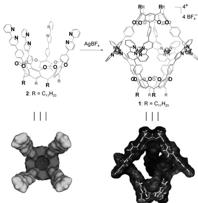
Scheme 1. Self-assembled capsule 1·4BF 4 and cavitaand 2 . In the energy-minimized structures, the long alkyl chains are omitted for viewing clarity. Van der Waals surfaces are shown in each structure. Left: Top view of the cavitaand. Right: Side view of the capsule. Some atoms have been removed to show the inner surface of the cavity.
