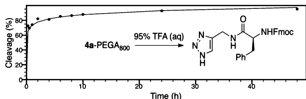
Figure 1. Acid-mediated release of triazole from 4a -PEGA 800 as a function of time.
