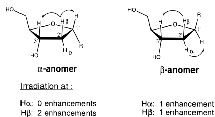
Figure 1. Illustration of qualitative differences in nuclear Overhauser enhancements observed for \alpha - (left) and \beta -anomers (right) of compounds 1–6. In \alpha -anomers, irradiation of the C-2'- \beta proton gives enhancements in both the C-1' and C-3' protons, while irradiation of the C-2'- \alpha proton gives little or no enhancement for either. In the \beta -anomers, irradiation of the C-2'- \beta proton gives enhancement only in the C-3' proton, while irradiation of the C-2'- \alpha proton gives enhancement only in the C-1' proton.
