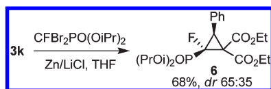
Scheme 3. Synthesis of Fluorinated Cyclopropyl Phosphonate 6
