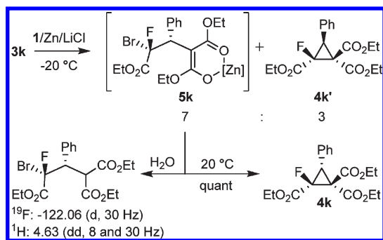
Scheme 2. Stepwise Cyclopropanation of Diethyl Benzyldene-malonate 3k
