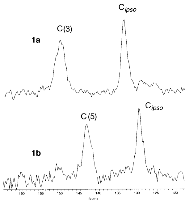
Fig. 1. Quaternary C-atoms obtained by means of the NQS sequence in 13 C-NMR CPMAS for desmotropes 1a and 1b
