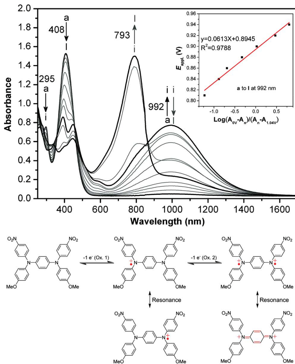
FIGURE 4 Absorption spectral change of compound M1 ( 5 \times 10^{-4} M) in 0.1 M TBAP/ \text{CH}_3\text{CN} at E_{\text{applied}} of (a) 0, (b) 0.81, (c) 0.84, (d) 0.86, (e) 0.88, (f) 0.90, (g) 0.92, (h) 0.94, (i) 1.00, (j) 1.03, (k) 1.06, and (l) 1.13 (V vs. Ag/AgCl) and the oxidation pathway. [Color figure can be viewed in the online issue, which is available at wileyonlinelibrary.com .]
