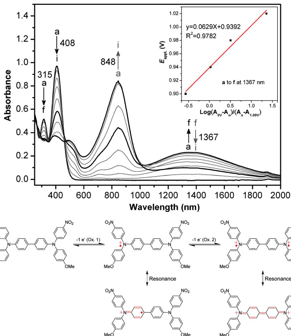
FIGURE 5 Absorption spectral change of compound M2 ( 5 \times 10^{-4} M) in 0.1 M TBAP/ \text{CH}_3\text{CN} at E_{\text{applied}} of (a) 0, (b) 0.90, (c) 0.94, (d) 0.98, (e) 1.02, (f) 1.04, (g) 1.06, (h) 1.09, and (i) 1.14 (V vs. Ag/AgCl) and the oxidation pathway. [Color figure can be viewed in the online issue, which is available at wileyonlinelibrary.com .]
