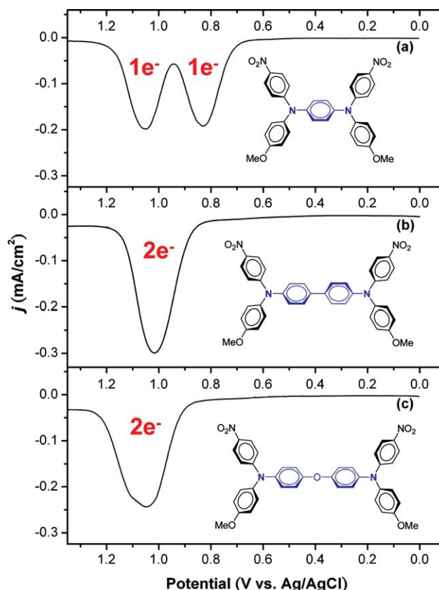
FIGURE 3 Differential pulse voltammograms of model compounds (a) M1 , (b) M2 , and (c) 2 ( 10^{-3} M) in 0.1 M TBAP/CH 3 CN at a scan rate of 50 mV/s. [Color figure can be viewed in the online issue, which is available at wileyonlinelibrary.com .]
