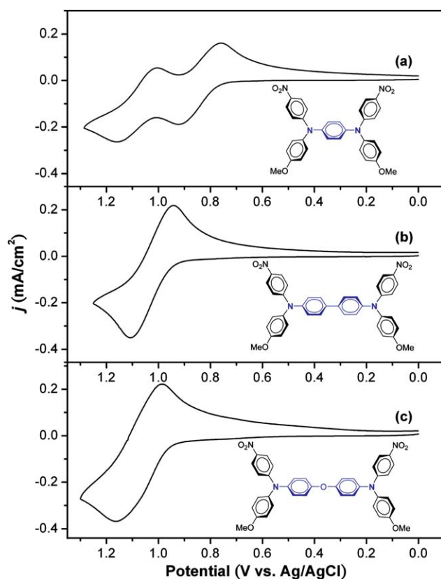
FIGURE 2 Cyclic voltammograms of 10^{-3} M model compounds (a) M1 , (b) M2 , and (c) 2 in 0.1 M TBAP/CH 3 CN at a scan rate of 50 mV/s. [Color figure can be viewed in the online issue, which is available at wileyonlinelibrary.com .]
