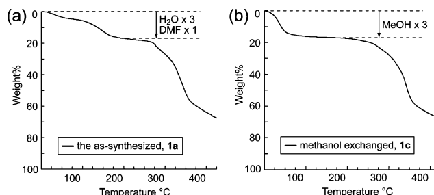
Figure 7. Thermogravimetric analyses of (a) 1a and (b) 1c over the temperature range from 25 to 450 \text{ }^\circ\text{C} at a heating rate of 10 \text{ }^\circ\text{C min}^{-1} under \text{N}_2 atmosphere. Amount of guests in figures is based on one 4-btapa ligand of each compound.
