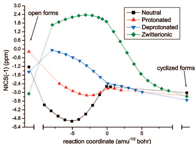
FIGURE 3. NICS values calculated along the IRC paths.
