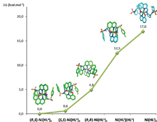
Figure 5. Relative Gibbs free energy for the most stable conformers calculated for octahedral nickel(II) complexes in methanol (from left to right): \Lambda\text{-C}(S,R)\text{N}(R,S)\text{-Ni}(\text{HL}^a)_2 , \Delta\text{-C}(S,S)\text{N}(R,R)\text{-Ni}(\text{HL}^a)_2 , \Delta\text{-C}(R,R)\text{N}(S,S)\text{-Ni}(\text{HL}^a)_2 , \text{Ni}(\text{HL}^a)(\text{HL}^i) , and \text{Ni}(\text{HL}^i)_2 (see also Supporting Information for more details). In the figure only the chirality of the N donor atom has been indicated to simplify and reduce the size of the labels.
