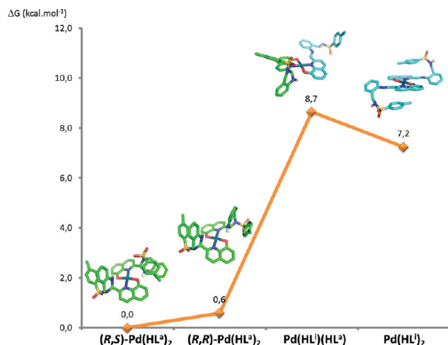
Figure 4. Relative Gibbs free energy for the most stable calculated conformers of (R,S)\text{-Pd}(\text{HL}^a)_2 , (R,R)\text{-Pd}(\text{HL}^a)_2 , \text{Pd}(\text{HL}^i)(\text{HL}^a) , and \text{Pd}(\text{HL}^i)_2 in methanol (left to right).
