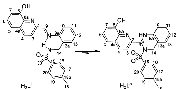
Scheme 1. Open-Chain Tautomer a H_2L^i en Route to the Final Thermodynamically Favored Amino Ring Tautomer H_2L^a
