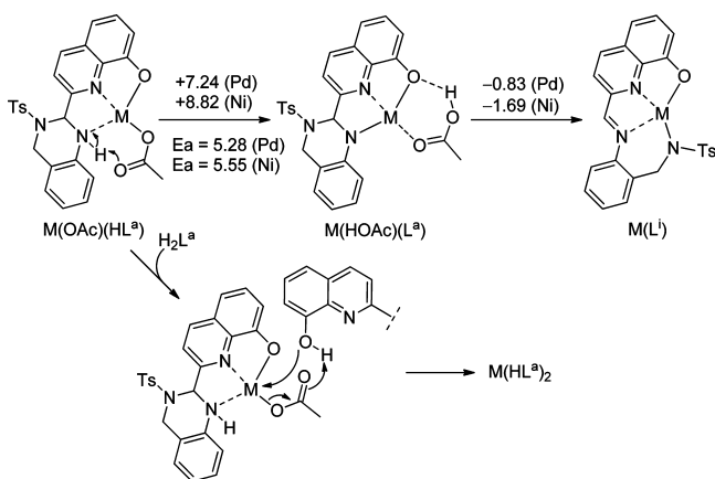
Scheme 4. General Proposed Mechanism for the Conversion of M(\text{OAc})(\text{HL}^a) to M(\text{L}^i) and M(\text{HL}^a)_2 a
