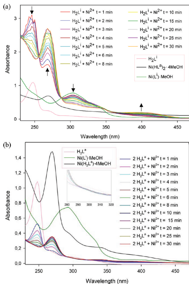
Figure 3. UV-vis spectroscopic monitoring of the reaction between \text{H}_2\text{L}^i/\text{H}_2\text{L}^a and \text{Ni}(\text{OAc})_2 \cdot 4\text{H}_2\text{O} (a) in 1:1 and (b) 2:1 molar ratios. Electronic spectra of \text{H}_2\text{L}^i/\text{H}_2\text{L}^a (pink line), \text{Ni}(\text{L}^i) \cdot \text{MeOH} (green line), and \text{Ni}(\text{HL}^a)_2 \cdot 4\text{MeOH} (black line) are included for comparison.
