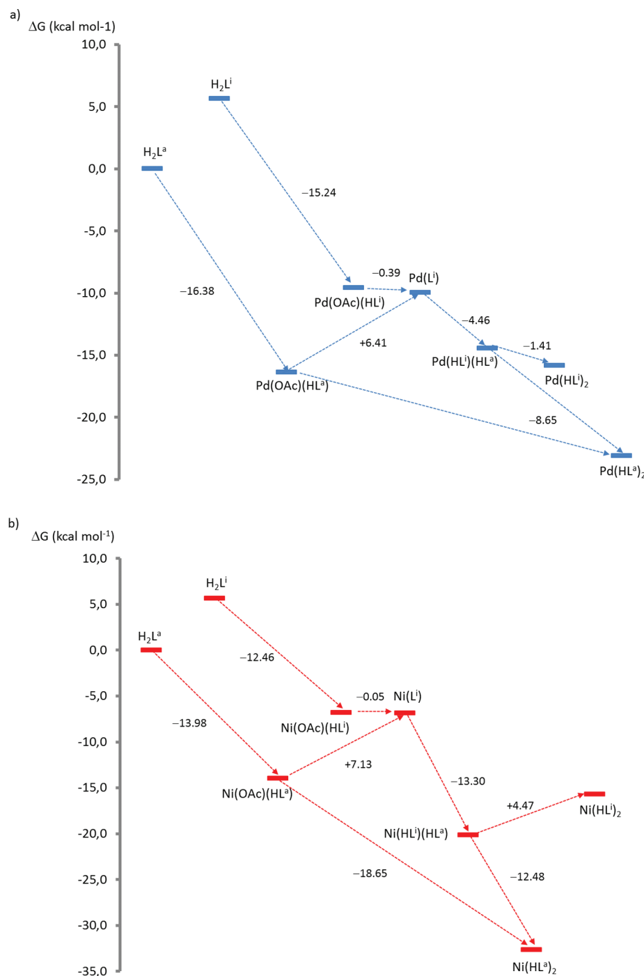
Figure 6. Complete Gibbs free energy profiles for the reactions between the closed-chain tetrahydroquinazoline H_2L^a and open-chain imine H_2L^i with (a) Pd(OAc)_2 \cdot 4H_2O and (b) Ni(OAc)_2 \cdot 4H_2O .
