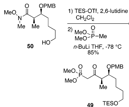
SCHEME 19. Synthesis of \beta -Ketophosphonate 49
