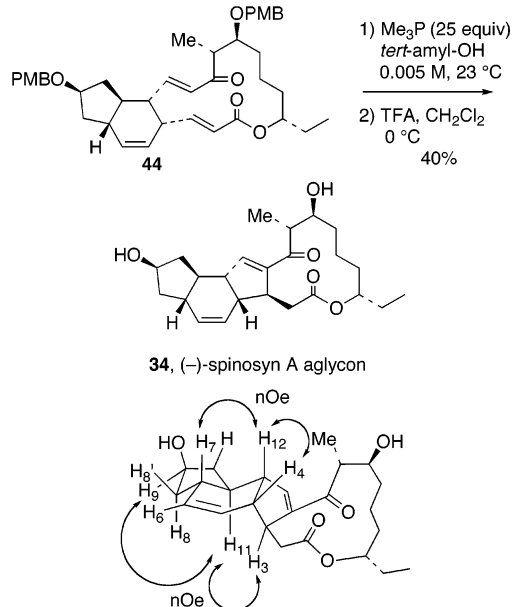
SCHEME 17. Synthesis of (–)-Spinosyn A Aglycon 34
