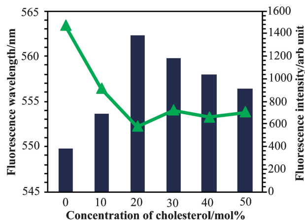
Figure 4. Fluorescence maximum ( \blacktriangle ) and intensity (peak height excited at the absorption maximum) ( \blacksquare ) of 1c in the PC vesicles with different CL concentrations. [1c]_{\text{final}} = 6.8 \mu\text{M} and [\text{lipid}]_{\text{total}} = 0.5 \text{ mM} . Excitation wavelength was 480 nm.
