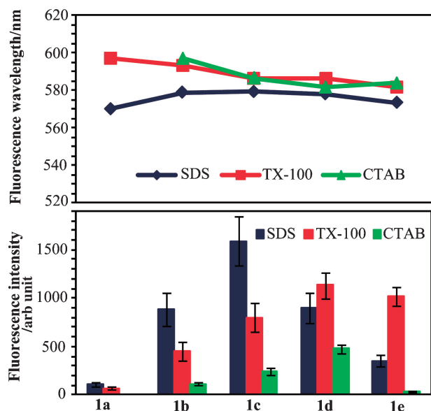
Figure 2. Fluorescence wavelength and intensity (peak height excited at the absorption maximum) of 1a–1e in three different micellar solutions. [1a-1e]_{\text{final}} = 6.8 \mu\text{M} , [\text{SDS}]_{\text{final}} = 50 \text{ mM} , [\text{TX-100}]_{\text{final}} = 1 \text{ mM} , and [\text{CTAB}]_{\text{final}} = 5 \text{ mM} . Error bars represent average \pm standard deviations of N = 3 independent experiments.
