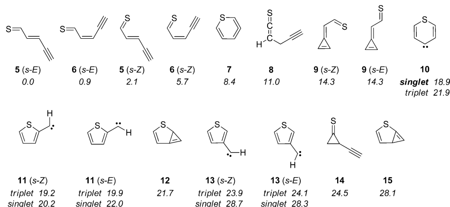
Scheme 2. C_5H_4S Isomers and Their Computed Relative Energies a
