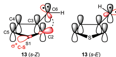
Figure 6. Natural Bond Orbital analysis of triplet 3-thienylcarbene (13).
