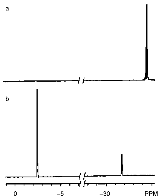
Fig. 2 ^{19}\text{F} NMR spectra of 9 (a) and 9 · \text{AgClO}_4 (b).
