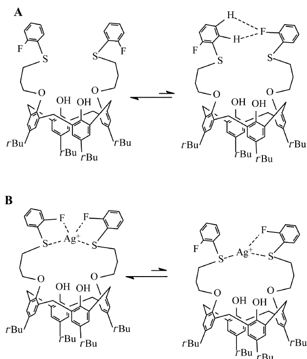
Chart 1 Conformational equilibria of 9 (A) and 9 · \text{AgClO}_4 (B).
