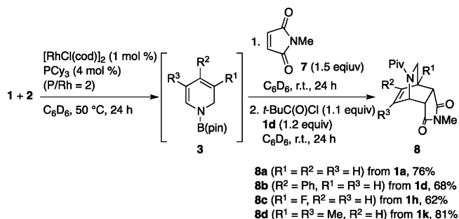
Scheme 3. Diels–Alder Reaction of N -Boryl-1,2-dihydropyridines
