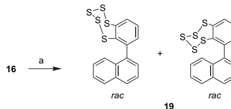
Scheme 6. (a) \text{S}_2\text{Cl}_2 (1.5 equiv)/ \text{BF}_3 \cdot \text{OEt}_2 , \text{CH}_2\text{Cl}_2 , rt, 1 h.
