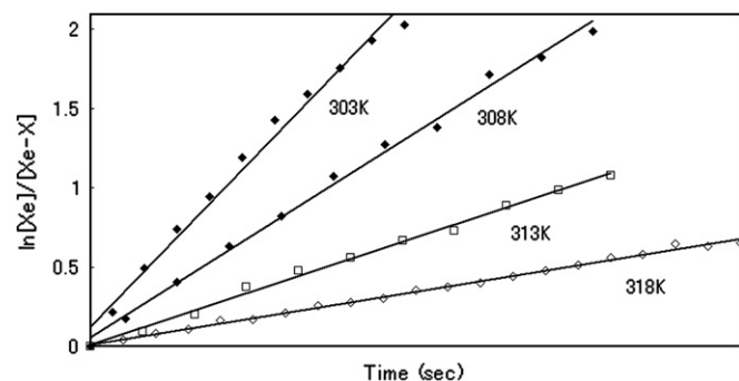
Figure 3. The representative kinetic data for the inversion of the pentathiepin ring of compound 19 ; [Xe]: equilibrium concentration; [Xe-X]: concentration as a function of time.
