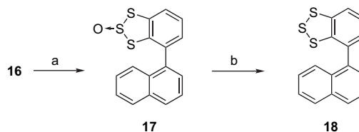
Scheme 5. (a) \text{SOCl}_2 /THF, rt, 0.5 h; (b) TMSOTf/THF, \text{SmI}_2 , -78\text{ °C} , 15 min.
