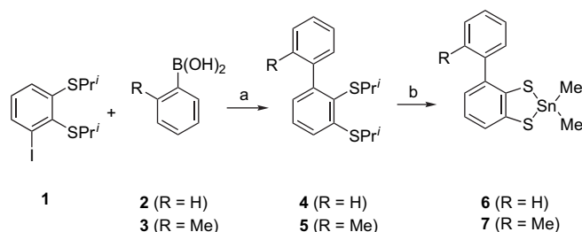
Scheme 1. (a) Pd(PPh 3 ) 4 (2 mol %), CsCO 3 (1 equiv), DMF/H 2 O, 120 °C, 6 h; (b) (i) Na (excess)/pyridine, reflux, 2 h, (ii) NaBH 4 /THF/EtOH, (iii) H 3 O + , (iv) Me 2 SnCl 2 .
