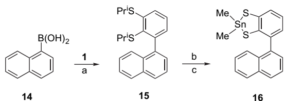
Scheme 4. (a) \text{Pd}(\text{PPh}_3)_4 (2 mol %), \text{CsCO}_3 (1 equiv), DMF/ \text{H}_2\text{O} , 120 °C, 6 h; (b) (i) Na (excess)/pyridine, reflux, 2 h, (ii) \text{NaBH}_4 /THF/EtOH, (iii) \text{H}_3\text{O}^+ ; (c) \text{Me}_2\text{SnCl}_2 .
