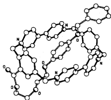
Fig. 3. A ball-and-stick representation of the X-ray crystal structure of self-complexing macrocycle 31 \cdot 4PF_6^- .
