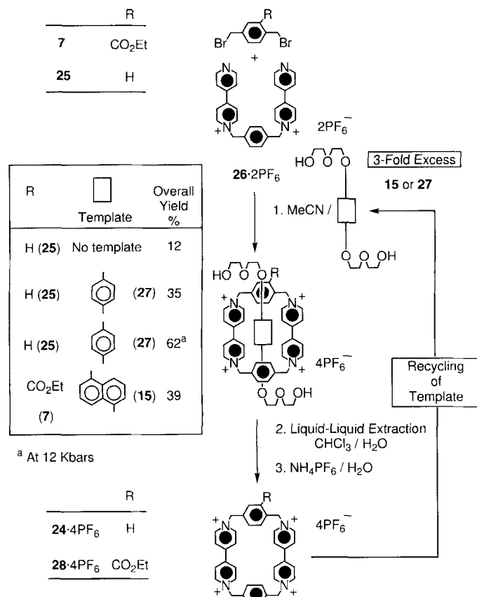
Scheme 7. The self-assembly of tetracationic cyclophanes 24 \cdot 4\text{PF}_6 and 28 \cdot 4\text{PF}_6 , assisted by noncovalent templates 15 and 27 .
