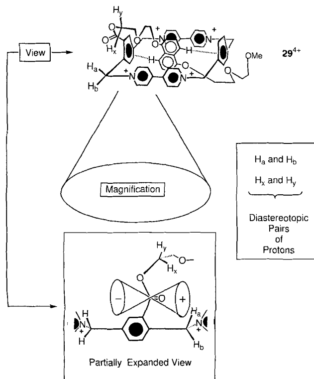
Fig. 6. A three-dimensional representation of the self-complexing conformation of 29-4PF 6 . The expanded view of the selected area reveals that the N -methylene protons and a proton belonging to \gamma -CH 2 O in the polyether chain are located within the deshielding environment of the anisotropic carbonyl group.
