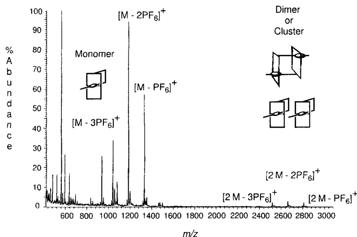
Fig. 4. Mass spectrum of the self-complexing macrocycle 29 \cdot 4\text{PF}_6 .
