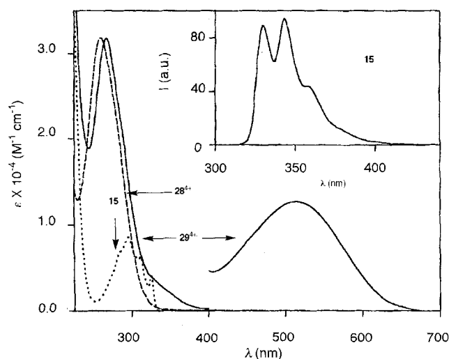
Fig. 10. Absorption spectrum of 29 4+ (unbroken line) and of its 28 4+ and 15 components. The fluorescence of 15 ( \lambda_{\text{exc}} = 295 \text{ nm} ) is shown in the inset.
