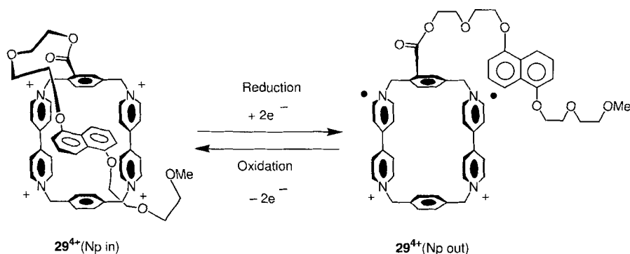
Fig. 15. Electrochemically driven dethreading–rethreading of 29^{4+} .
