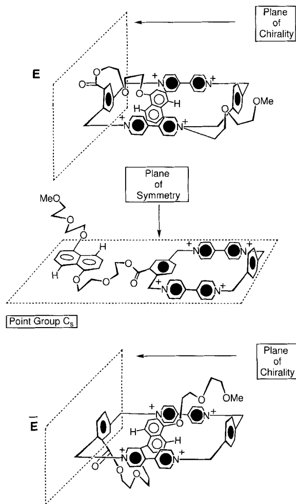
Scheme 10. A representation of the two possible enantiomeric forms for a self-complexing macrocycle 29 + PF 6 - and of the unthreaded intermediate possessing a plane of symmetry.
