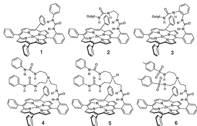
Figure 1. Porphyrin hosts.
