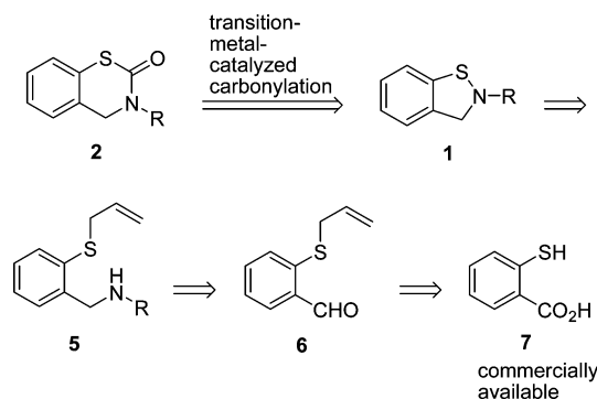
FIGURE 1. Retrosynthetic analysis.
