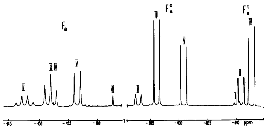
Fig. 2. ^{19}\text{F} NMR spectrum (75.39 MHz) for \text{K}_2[\text{RuNOF}_5] \cdot 2\text{H}_2\text{O} solution in concentrated ( \sim 40\% ) \text{HClO}_4 at 10^\circ\text{C} .
