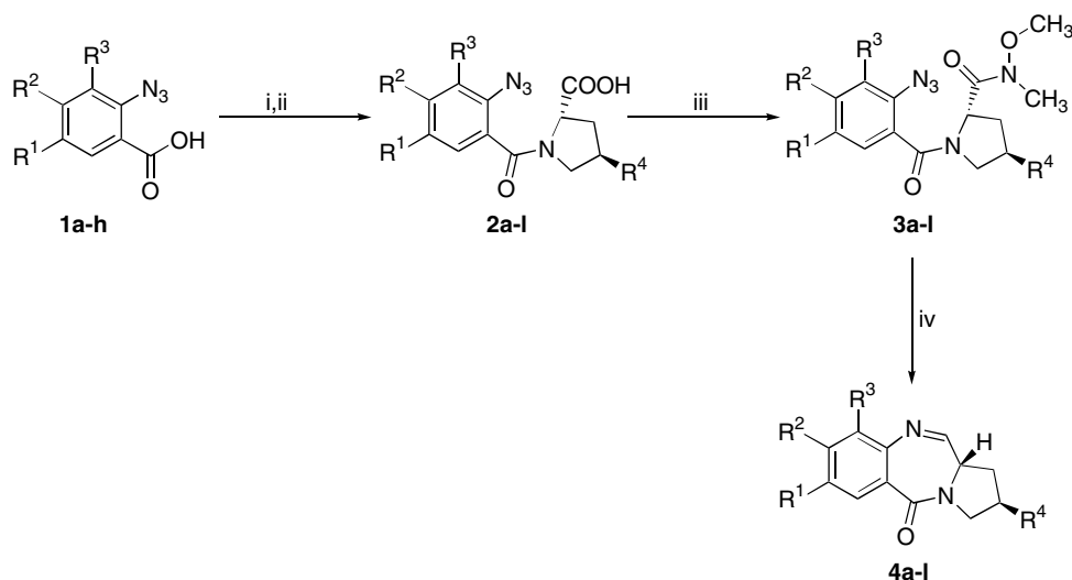
Scheme 1. Reagents and conditions: (i) (\text{COCl})_2 , 1–3 drops DMF, \text{CH}_2\text{Cl}_2 , 0^\circ\text{C} –rt, 2 h; (ii) \text{Et}_3\text{N} , L -proline hydrochloride or hydroxy L -proline hydrochloride, THF/ \text{H}_2\text{O} , 0^\circ\text{C} –rt, 2 h, 75–80%; (iii) N,O -dimethylhydroxylamine hydrochloride, EDCI, NMM, \text{CH}_2\text{Cl}_2 , -15^\circ\text{C} , 1 h, 80–85%; (iv) \text{LiAlH}_4 , dry THF, -15 to -20^\circ\text{C} , 40–50 min or \text{LiBH}_4 dry THF 0^\circ\text{C} –rt, 120–140 min, 50–68%.
