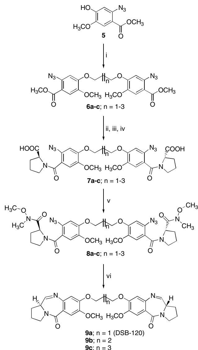
Scheme 2. Reagents and conditions: (i) \text{K}_2\text{CO}_3 , dibromoalkane, dry DMF, rt, 12 h, 85%; (ii) \text{LiOH} (2 N) THF/MeOH/ \text{H}_2\text{O} (3:1:1), rt, 4 h, 85–88%; (iii) (\text{COCl})_2 , 1–3 drops DMF, \text{CH}_2\text{Cl}_2 , 0 °C–rt, 2 h; (iv) \text{Et}_3\text{N} , L -proline hydrochloride, THF/ \text{H}_2\text{O} , 0 °C–rt, 2 h, 75%; (v) N,O -dimethylhydroxylamine hydrochloride, EDCI, NMM, \text{CH}_2\text{Cl}_2 , –15 °C, 1 h, 85%; (vi) \text{LiAlH}_4 , dry THF, –15 to –20 °C, 40–50 min or \text{LiBH}_4 dry THF 0 °C–rt, 120–140 min, 50–68%.
