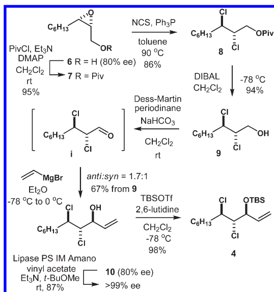
Scheme 2. Synthesis of C12–C22 Fragment 4
