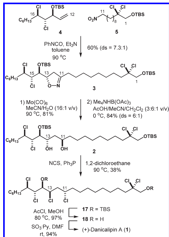
Scheme 4. Completion of Total Synthesis of (+)-Danicalipin A via 1,3-Dipolar Coupling between C1–C11 Fragment 5 and C12–C22 Fragment 4
