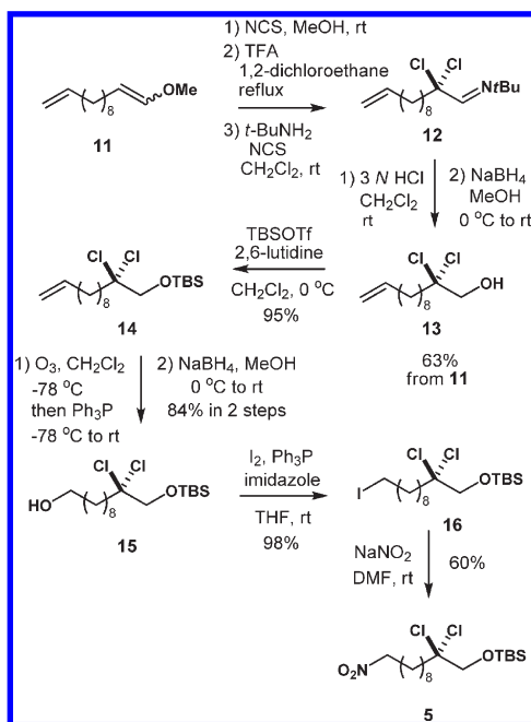
Scheme 3. Synthesis of C1–C11 Fragment 5
