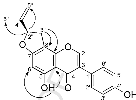
Fig. 1. Structure of derrisisoflavone G ( 1 ) with key HMBC (H → C) correlations.
