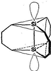
Fig. 1. A strain-relieved model of 1,6-disila[4.4.4]propellane with two trigonal-bipyramidal silicon atoms.
