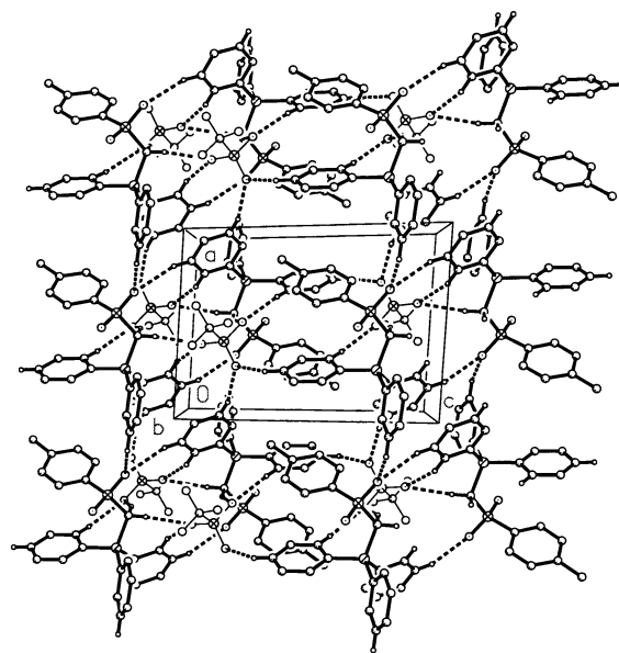
Figure 2. Packing diagram showing hydrogen bond interactions in [\text{4-MeC}_6\text{H}_4\text{S}(\text{O})_2\text{CH}_2\text{PPh}_3]\text{TfO} .
