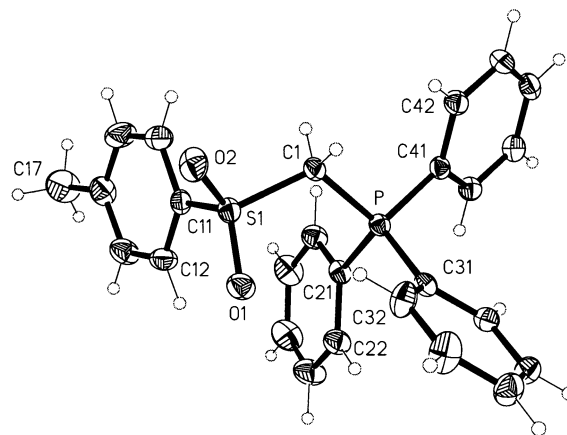
Figure 1. Thermal ellipsoid plot of the cation [\text{4-MeC}_6\text{H}_4\text{S}(\text{O})_2\text{CH}_2\text{PPh}_3]^+ (50% probability level) with the labeling scheme. Selected bond lengths (Å) and angles (deg): \text{P}-\text{C}(41) = 1.7927(18) , \text{P}-\text{C}(21) = 1.7932(18) , \text{P}-\text{C}(31) = 1.7935(19) , \text{P}-\text{C}(1) = 1.8145(18) , \text{S}(1)-\text{O}(1) = 1.4358(14) , \text{S}(1)-\text{O}(2) = 1.4385(14) , \text{S}(1)-\text{C}(11) = 1.7549(19) , \text{S}(1)-\text{C}(1) = 1.7968(18) , \text{S}(2)-\text{O}(5) = 1.426(2) , \text{S}(2)-\text{O}(3) = 1.428(3) , \text{S}(2)-\text{O}(4) = 1.429(2) , \text{S}(2)-\text{C}(99) = 1.809(3) , \text{C}(99)-\text{F}(1) = 1.306(4) , \text{C}(99)-\text{F}(3) = 1.311(3) , \text{C}(99)-\text{F}(2) = 1.329(4) ; \text{C}(41)-\text{P}-\text{C}(21) = 107.90(9) , \text{C}(41)-\text{P}-\text{C}(31) = 110.13(8) , \text{C}(21)-\text{P}-\text{C}(31) = 110.07(9) , \text{C}(41)-\text{P}-\text{C}(1) = 106.37(8) , \text{C}(21)-\text{P}-\text{C}(1) = 110.95(8) , \text{C}(31)-\text{P}-\text{C}(1) = 111.31(9) , \text{O}(1)-\text{S}(1)-\text{O}(2) = 119.45(9) , \text{O}(1)-\text{S}(1)-\text{C}(11) = 108.71(9) , \text{O}(2)-\text{S}(1)-\text{C}(11) = 107.68(9) , \text{O}(1)-\text{S}(1)-\text{C}(1) = 108.33(8) , \text{O}(2)-\text{S}(1)-\text{C}(1) = 105.05(8) , \text{C}(11)-\text{S}(1)-\text{C}(1) = 106.98(9) , \text{S}(1)-\text{C}(1)-\text{P} = 116.42(10) .
