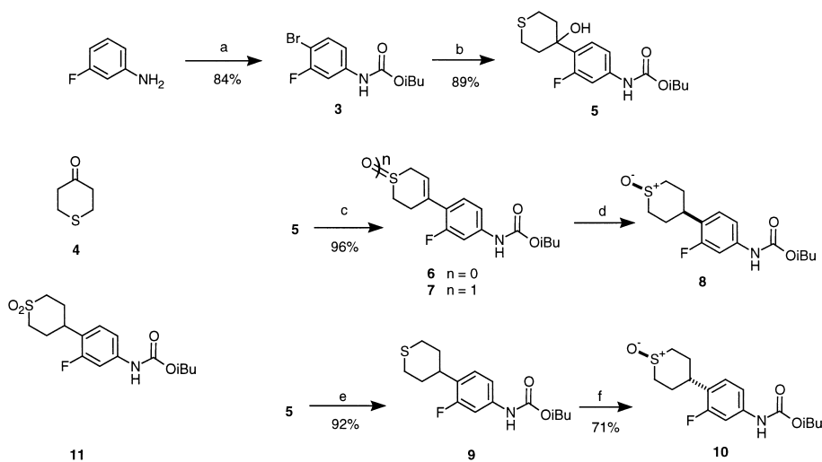
Scheme 2. Reagents and conditions: (a) isobutylchloroformate, \text{K}_2\text{CO}_3 , \text{CH}_2\text{Cl}_2/\text{water} , 1,3-dibromo-5,5-dimethylhydantoin; (b) EtMgBr, n -BuLi, MgBrCl, THF, then 4 ; (c) TFA, \text{CH}_2\text{Cl}_2 , \text{NaIO}_4 , MeOH/water; (d) 5% Pt/C, \text{H}_2 , DMF; (e) (\text{Me}_3\text{Si})_2\text{O} , PMHS, p TSA, toluene; (f) \text{Ti}(\text{OiPr})_4 , D-diisopropyl tartrate, t BuOOH, \text{CH}_2\text{Cl}_2
