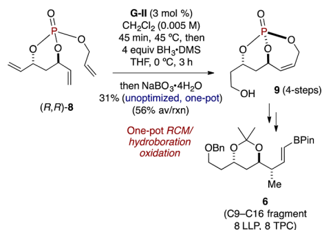
Scheme 2. One-Pot, Sequential RCM/ \text{BH}_3\cdot(\text{ox}) Protocol
