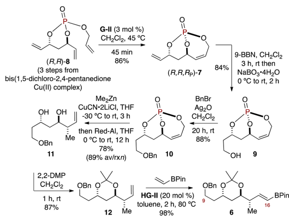
Scheme 1. Synthesis of the C9–C16 Fragment
