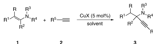
Scheme 1. Synthesis of propargylamines of type 3 by the addition of alkynes 2 to enamines 1 .
