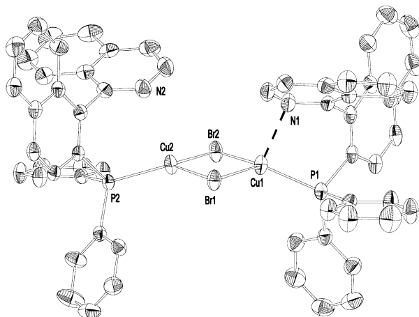
Figure 2. Structure of the complex [\text{BrCu}(\text{Quinap})]_2 ( 11 ) in the solid state (the hydrogen atoms and crystallized solvent molecules are omitted for clarity). Selected bond lengths [Å] and angles [°]: Cu1–Br1 2.4728(8), Cu2–Br2 2.4150(8), Cu1–P1 2.199(2), Cu2–P2 2.1827(13); P2–Cu2–Br2 129.28(4), P2–Cu2–Br1 122.75(4), Br2–Cu2–Br1 104.18(3).
