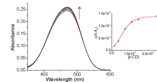
Figure 3. Absorbance spectra of L (4.23 μM) with varying [\beta\text{-CD}] (0–0.247 mM) in a \text{CH}_3\text{CN} -aq. HEPES buffer (0.01 M, pH 7.2; 2:3, v/v). Inset: plot of change in absorbance ( A - A_0 ) of L against varied concentrations of β-CD.
