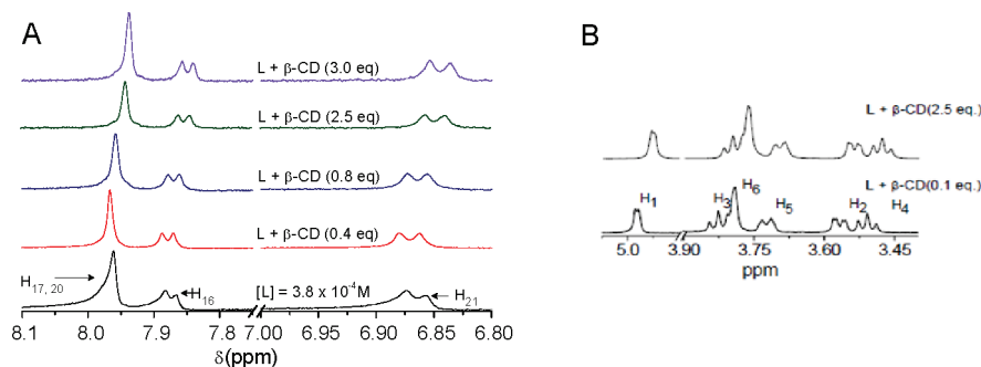
Figure 2. (A) Partial ^1\text{H} NMR spectra of L (8 mM) with varying [\beta\text{-CD}] (0–15.2 mM; in \text{CD}_3\text{CN}-\text{D}_2\text{O} , 1:1, v/v). (B) Partial ^1\text{H} NMR spectra of L · 2β-CD for \delta = 3.45\text{--}5 ppm, a region where L does not have any resonance signal.
