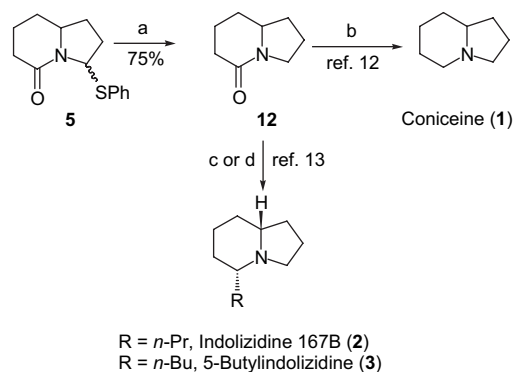
Scheme 4. Synthesis of indolizidine alkaloids 1 – 3 . Reagents and conditions: (a) n -Bu 3 SnH (2.5 equiv), AIBN (0.3 equiv), toluene, reflux 20 h; (b) LiAlH 4 (2.54 equiv), THF, reflux 15 h; (c) (i) n -PrMgBr (3 equiv), THF, 0 °C to rt, 4 h; (ii) AcOH then NaBH 4 (2 equiv), 0 °C, 1 h; (d) (i) n -BuMgCl (3 equiv), THF, 0 °C to rt, 4 h; (ii) AcOH then NaBH 4 (2 equiv), 0 °C, 1 h.
