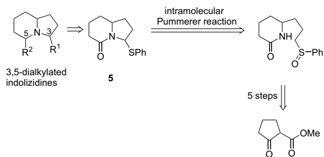
Scheme 2. Synthetic strategy.
