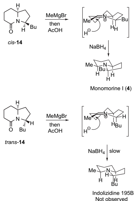
Scheme 6.
