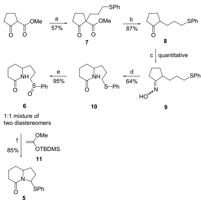
Scheme 3. Reagents and conditions: (a) (i) NaH (1.2 equiv), DMF, 1,3-dibromopropane (3 equiv), rt, 20 h; (ii) PhSH (1.05 equiv), Et 3 N (1.25 equiv), THF, 0 °C to rt, 24 h; (b) NaCN (1.2 equiv), DMSO, 160 °C, 3 h; (c) NH 2 OH·HCl (1.2 equiv), NaOAc (1.73 equiv), aq EtOH; (d) 1 N NaOH (1.1 equiv), PhSO 2 Cl (1.1 equiv), acetone, rt, 24 h; (e) NaIO 4 (1.15 equiv), aq MeOH, 0 °C to rt, 24 h; (f) ZnI 2 (10 mol %), 11 (2 equiv), CH 3 CN, rt, 24 h.
