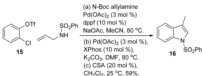
Scheme 7. Use of Benzenesulfonyl Allylamine
