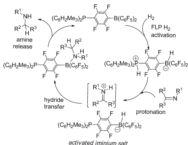
Scheme 3. Proposed Mechanism of Hydrogenation
