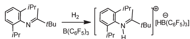
Scheme 4. Hydrogenation of Sterically Encumbered Imine
