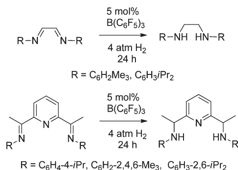
Scheme 6. Reduction of Diimines
