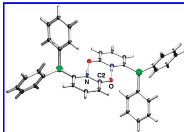
Figure 3. X-ray structure of the symmetric dimer 4A of 6-DPPon ( 2 ).
