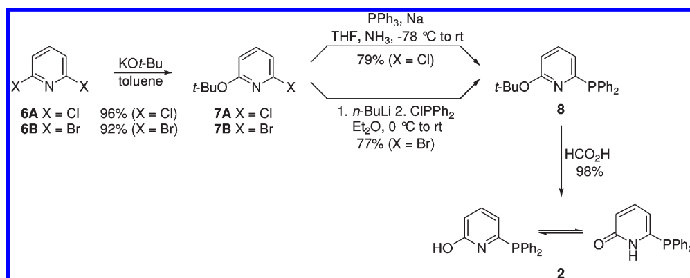
Scheme 4. Alternative Preparation of 6-DPPon (2) via a Nucleophilic (Upper Pathway) or Electrophilic Aromatic (Lower Pathway) Displacement
