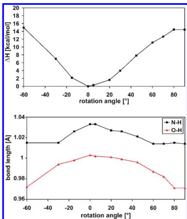
Figure 8. Rotation of pyridone and hydroxypyridine rings from the equilibrium structure. (Top) Change of total energy. (Bottom) Change of N–H and O–H bond lengths.
