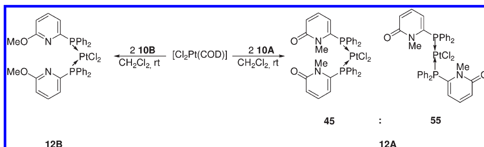
Scheme 9. Synthesis of the Pt Complexes Bearing the Fixed Tautomers of 2
