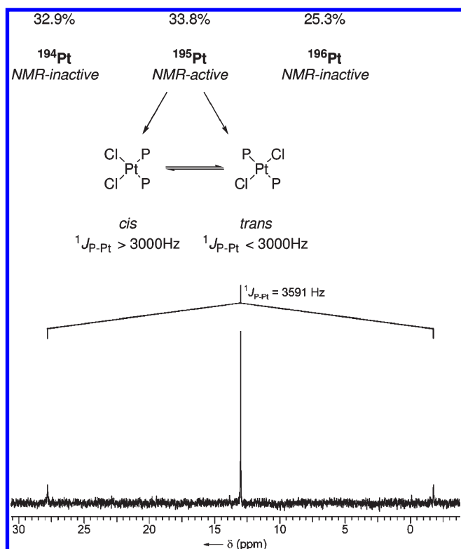
Figure 5. Coupling in complexes of the general type [\text{Cl}_2\text{PtP}_2] (top) and ^{31}\text{P} NMR spectrum for [\text{Cl}_2\text{Pt}(\text{6-DPPon})_2] (bottom).
