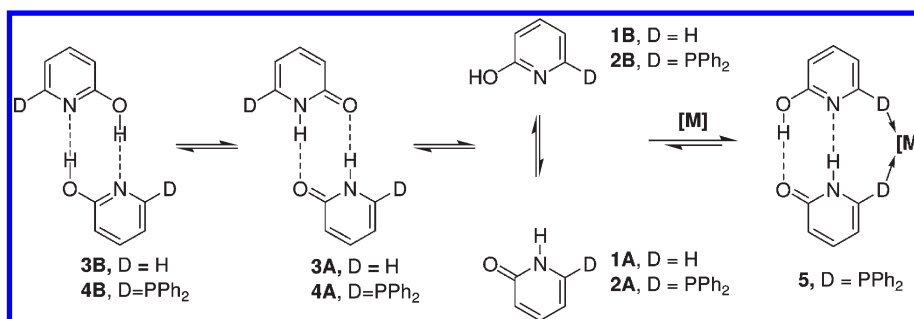
Scheme 2. Self-Assembling of the 6-DPPon Ligand in the Presence of a Transition Metal Center
