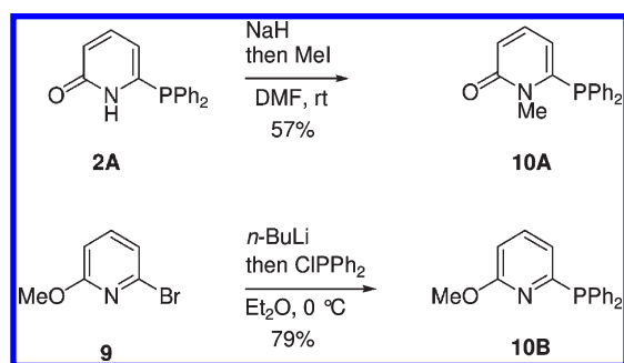
Scheme 5. Preparation of Methyl-Fixed Tautomers 10A (6-DPMePon) and 10B (2-MeODPP)
