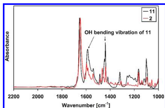
Figure 11. Direct comparison between the IR spectra of 2 and 11.
