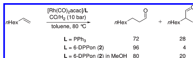
Scheme 3. Rhodium-Catalyzed Hydroformylation of 1-Octene: Complementary Behavior of PPh_3 and 2 a
