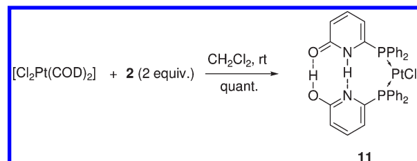
Scheme 7. Preparation of cis - [\text{Cl}_2\text{Pt}(\text{6-DPPon})_2] Complex 11
