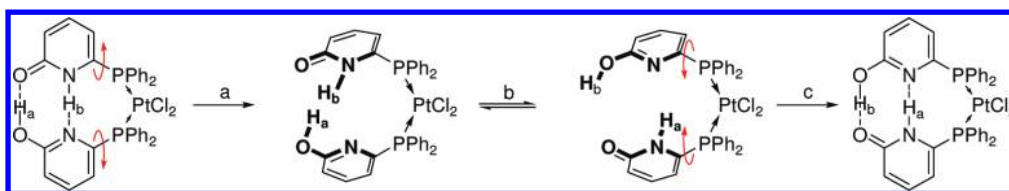
Scheme 8. Process That Renders the Hydrogen Bonds Indistinguishable: (a) Rotation along the C α –P Bond, (b) Intramolecular Tautomerism, and (c) Rotation Back in Plane and Formation of the Hydrogen Bonds
