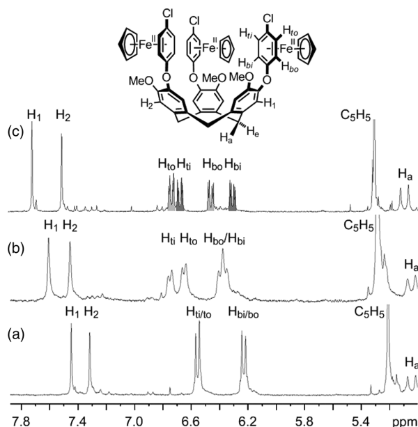
Figure 5. The 1 H NMR spectrum of (±)- 2d [PF 6 ] 3 in (a) NO 2 Me- d 3 , (b) NO 2 Me- d 3 with excess added [NBu 4 ]Br and (c) acetone- d 6 , highlighting the peak splitting that occurs upon anion binding.
