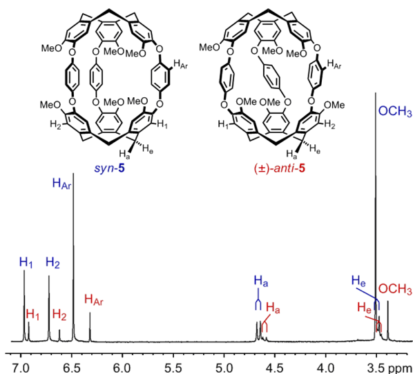
Figure 4. 1 H NMR spectrum (400 MHz, CDCl 3 ) of an approximate 5:1 mixture of syn - 5 and (±) - anti - 5 .
