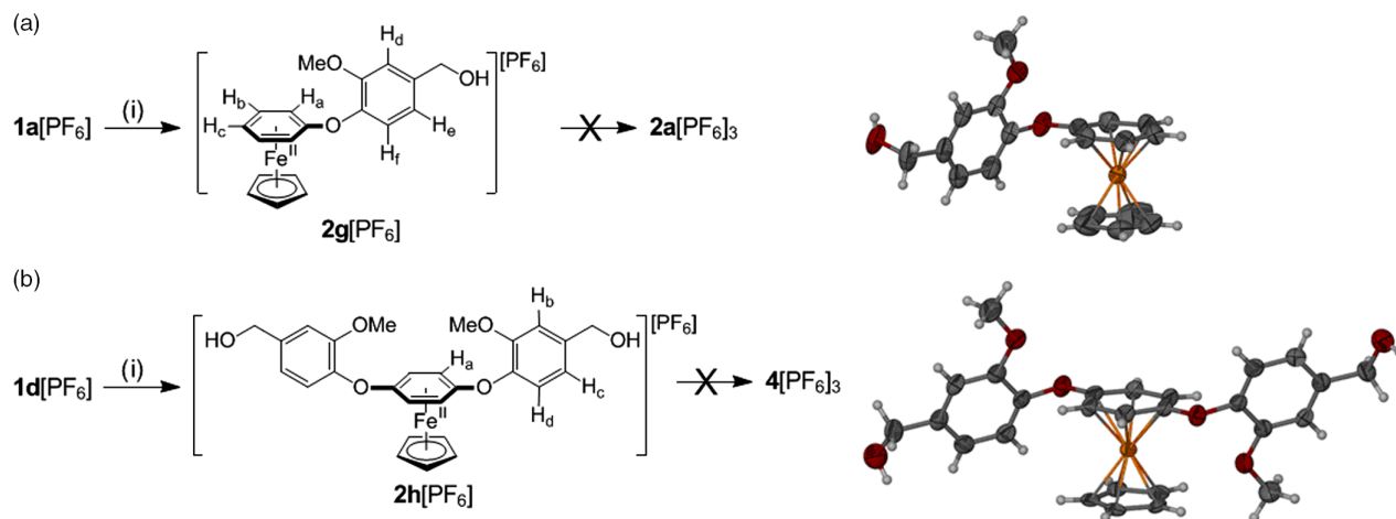
Figure 3. Synthesis of potential CTB and cryptophane precursors 2g[PF_6] and 2h[PF_6] : (i) K_2CO_3 , DMF, excess vanillyl alcohol. Thermal ellipsoid plots of the cations from the X-ray crystal structures of (a) 2g[PF_6] and (b) 2h[PF_6] -DMF. The [(\eta^5-C_5H_5)Fe^{II}]^+ moiety of 2h^+ is disordered about the two faces of the coordinated arene. Only the major occupancy portion (80%) is shown.
