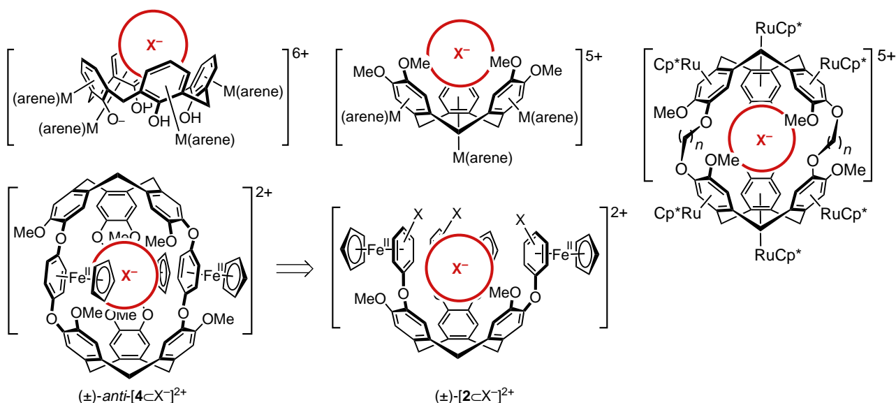
Scheme 2. Anion-binding, organometallic cavitands and cryptophanes.
