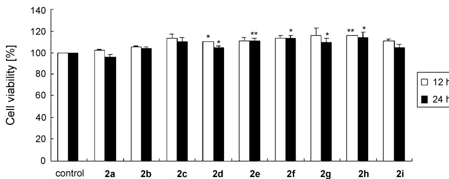
Fig. 3. Effects of compounds 2a–2i on cell viability of VECs at the concentration of 2.5 \mu\text{M} for 12 and 24 h (*: p < 0.05 , **: p < 0.01 vs. control group, n = 3 )
