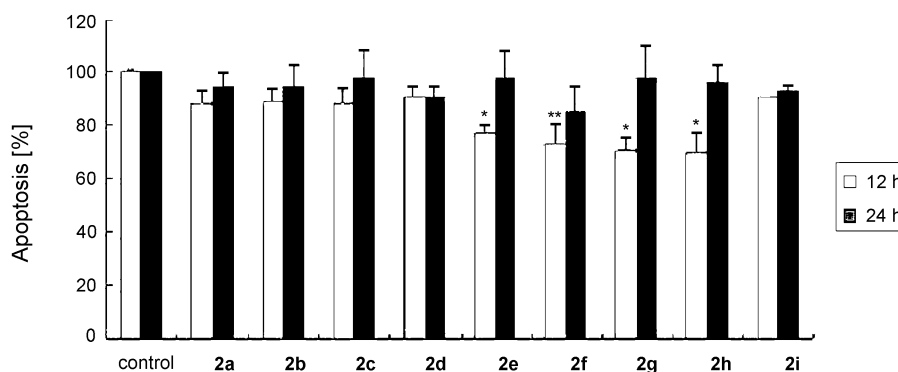
Fig. 4. Inhibition of VEC apoptosis by compounds 2a–2i at the concentration of 2.5\ \mu\text{M} for 12 and 24 h. Ratio of apoptotic cells vs. control. Results are presented as mean \pm SE ( n = 3 , *: P < 0.05 vs. control, **: P < 0.01 vs. control).
