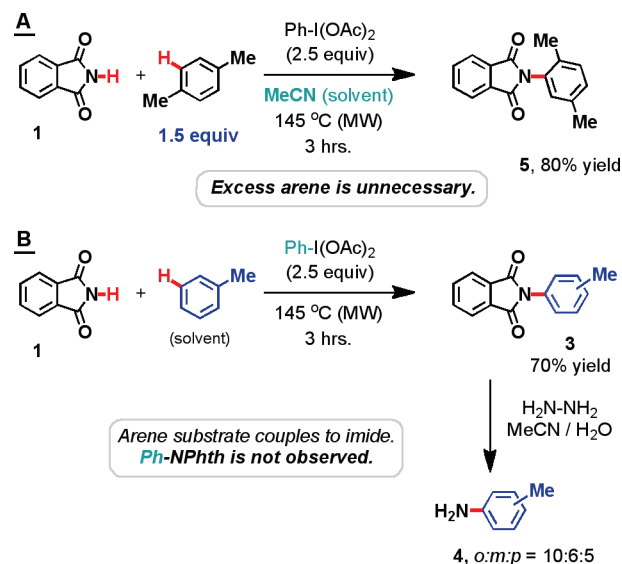
Scheme 1. Oxidative Amination of Substituted Arenes
