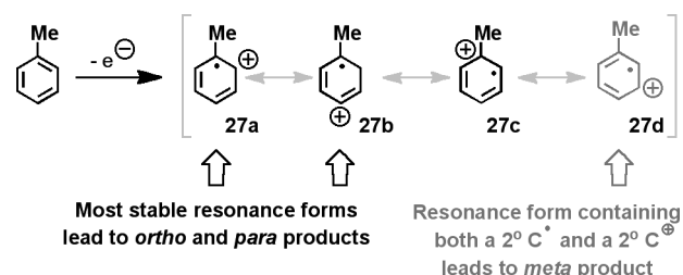
Scheme 3. Resonance Structures of the Aryl Radical Cation Explain the Observed Regioselectivities
