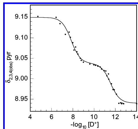
Figure 1. Data points are the observed limiting fast exchange mole fraction averaged pyrrole ^1\text{H} NMR chemical shifts for compounds 2 , 3 , and 4 in \text{D}_2\text{O} as a function of -\log_{10}[\text{D}^+] . The solid line is the nonlinear least-squares best fit line giving K_1(298\text{ K}) = (1.40 \pm 0.2) \times 10^{-8} , K_2(298\text{ K}) = (2.8 \pm 0.3) \times 10^{-12} , and \delta_3(\text{pyr}) = 9.04\text{ ppm} ; 2 is [(\text{TSPP})\text{Rh}^{\text{III}}(\text{D}_2\text{O})_2]^{-3} , \delta_2(\text{pyr}) = 9.15\text{ ppm} ; 4 is [(\text{TSPP})\text{Rh}^{\text{III}}(\text{OD})_2]^{-5} , \delta_4(\text{pyr}) = 8.94\text{ ppm} ; 3 is [(\text{TSPP})\text{Rh}^{\text{III}}(\text{D}_2\text{O})(\text{OD})]^{-4} .
