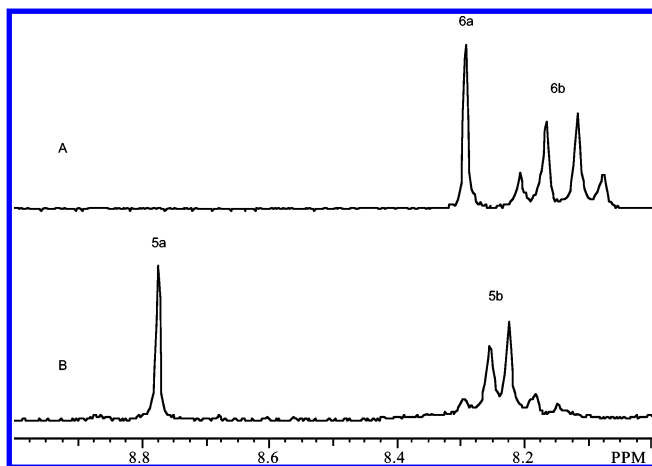
Figure 2. 1 H NMR (360 MHz) spectra in D 2 O. (A) [(TSPP)Rh I (D 2 O)] -5 ( 6 ) in D 2 O, [D + ] < 10 -10 M, T = 298 K; (B) [(TSPP)Rh I -D(D 2 O)] -4 ( 5 ), [D + ] < 10 -4 M, T = 360 K. a, pyrrole hydrogens; b, phenyl hydrogens.
