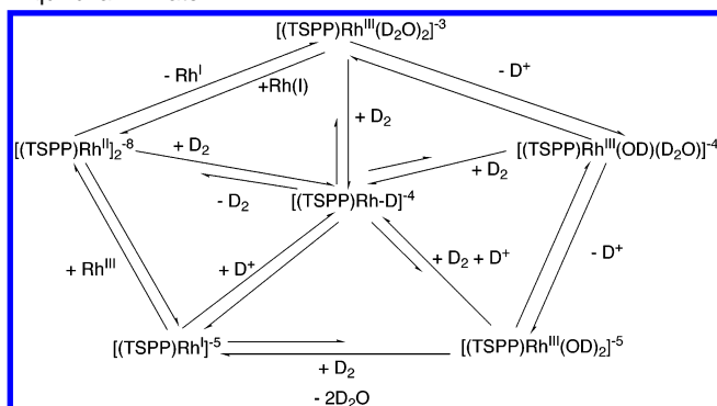
Scheme 1. The (TSPP)Rh Species in Simultaneous Multiple Equilibria in Water
