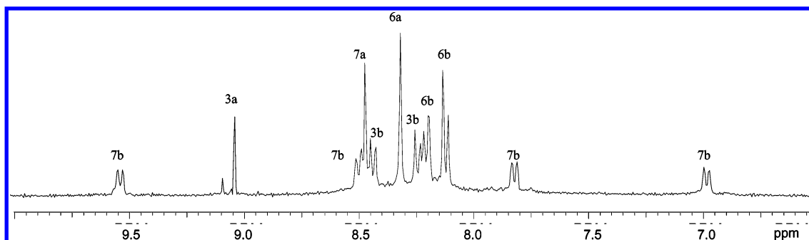
Figure 4. ^1\text{H} NMR (360 MHz) spectrum of [(\text{TSPP})\text{Rh}^{\text{II}}(\text{D}_2\text{O})_2]_2^{-8} ( 7 ) in equilibrium with [(\text{TSPP})\text{Rh}^{\text{I}}]^{-5} ( 6 ) and (TSPP)Rh(III) species 2 and 3 in \text{D}_2\text{O} ( [\text{D}^+] = 10^{-8} M), where a and b designated the pyrrole and phenyl hydrogens, respectively, in species 3 , 6 , and 7 .
