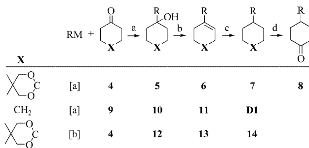
Scheme 2. Syntheses of ketone 8 , D1 , and 14 . Conditions/reagents: (a) THF; (b) for 5 and 12 : p -toluenesulfonic acid, toluene; for 10 : CF 3 COOH; (c) 1 atm. H 2 , Pd/C, THF/EtOH; (d) HCl, H 2 O/THF
