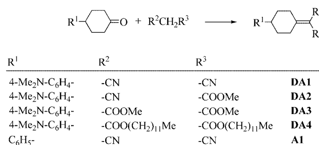
Scheme 3. Synthesis of D–σ–A compounds and model acceptor compound A1 . Conditions/reagents for DA1 , DA2 , and A1 : β-alanine, EtOH/H 2 O; for DA3 and DA4 : TiCl 4 , pyridine, THF
