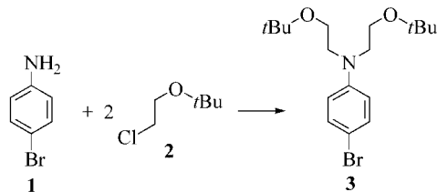
Scheme 1. Synthesis of 3 . Conditions/reagents: K 2 CO 3 , KI, butanol
