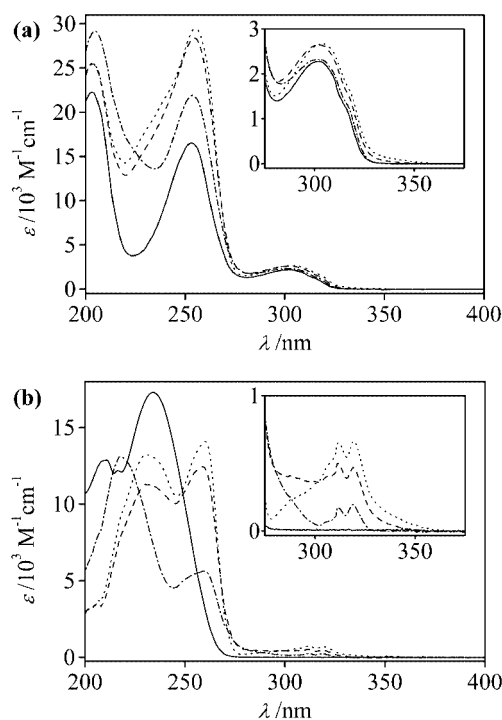
Figure 2. (a) Absorption spectra of D1 (—), DA1 (···), DA2 (— — —), and DA3 (— · —) in cyclohexane at 20 °C. The inset shows a magnification of the region 275–375 nm. (b) Absorption spectrum of A1 (—) in cyclohexane at 20 °C and difference spectra obtained upon subtraction of the absorption spectrum of D1 from that of DA1 (···), DA2 (— — —) and DA3 (— · —). The inset shows a magnification of the region 275–375 nm
