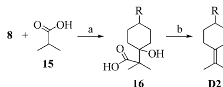
Scheme 4. Synthesis of D2 (R = 4-Me 2 NC 6 H 4 -). Conditions/reagents: (a) LDA, THF; (b) Me 2 NCH(OCH 2 t Bu) 2 , MeCN
