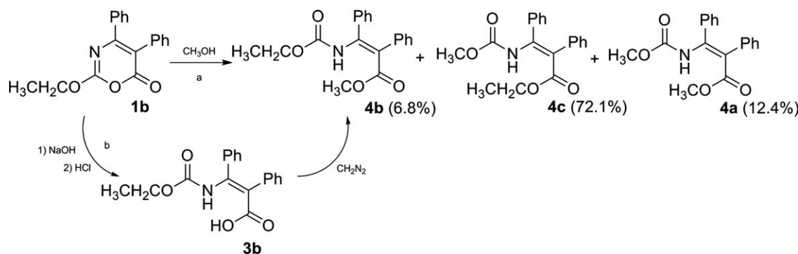
Scheme 3. Reaction of compound 1b with methanol.
