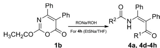
Scheme 4. Reaction of compound 1b with sodium alkoxide and sodium ethanethiolate.
