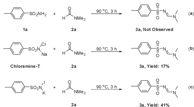
Scheme 1. Preliminary Test for N -Sulfonyl Formamide Synthesis
