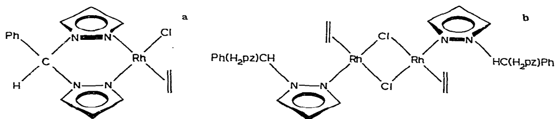
Fig. 2. Possible structures for [(\text{LL})\text{Rh}(\text{C}_2\text{H}_4)\text{Cl}]_x .
