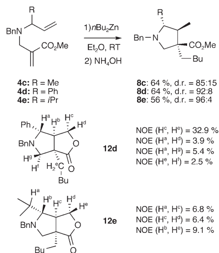
Scheme 5. Domino reactions with enoates 4c–e .
