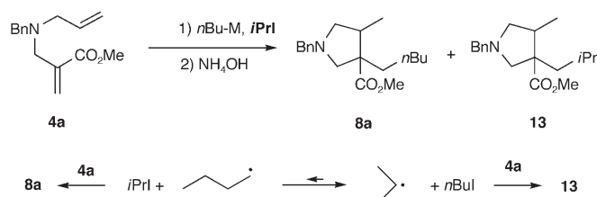
Scheme 6. Scrambling experiments.
