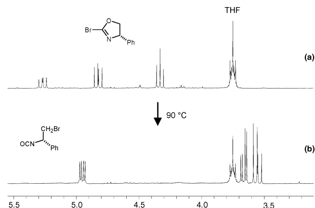
Figure 1. ^1\text{H} NMR spectra ( \text{CDCl}_3 , 300 MHz) of (a) (4 R )-2-bromo-4-phenyloxazoline 1c ; (b) after heating 90\text{ }^{\circ}\text{C} for 2 days.
