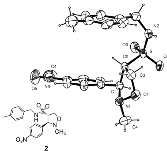
Figure 1. 2-Methyl-3-(4-nitro-phenyl)-isoxazolidine-4-sulfonic acid 4-methyl-benzamide.
