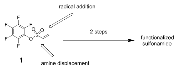
Scheme 1. Previously Described Strategy for Sulfonamide Formation
