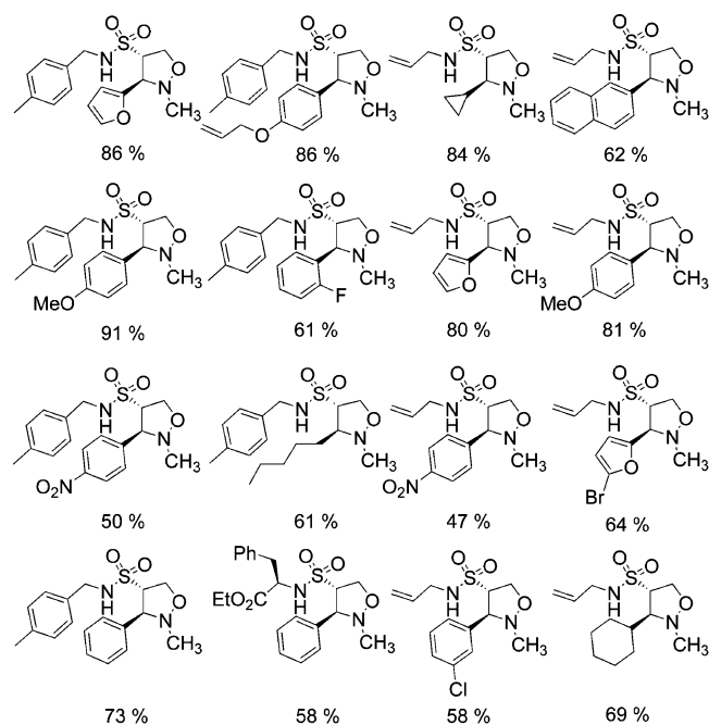
Figure 2. Isoxazolidine sulfonamides formed from PFP-substituted cycloadducts via aminolysis.
