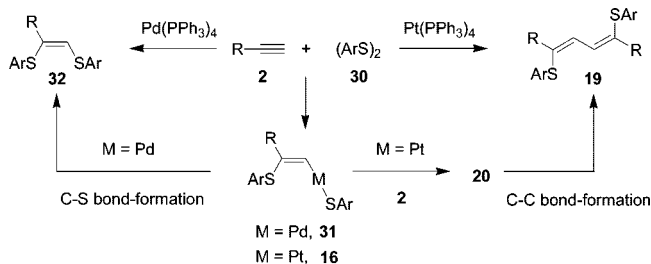
Scheme 12. Pd-Catalyzed vs Pt-Catalyzed Reaction of 2 with 30
