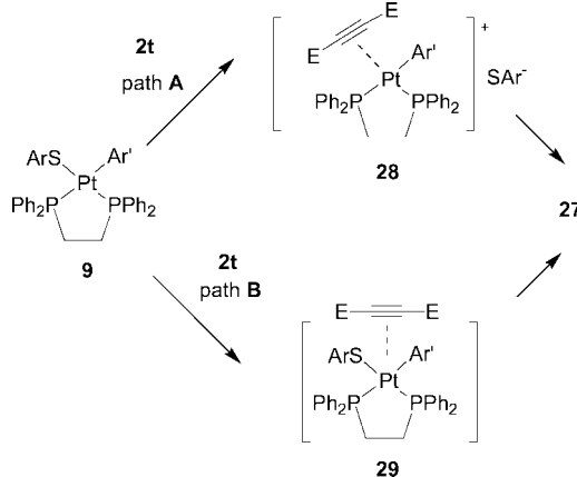
Scheme 10. Plausible Reaction Pathways for the Insertion of 2t into the S–Pt Bond of 9
