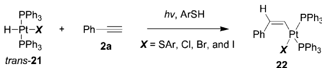
Scheme 7. Photo- and Thiol-Driven trans -Insertion of Phenylacetylene ( 2a ) into the H–Pt Bond of trans -Pt(H)(X)-(PPh 3 ) 2 ( 21 ) 42
