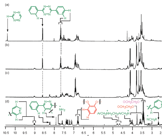
Figure 4. 1 H NMR spectra (400 MHz, CD 3 CN, 298 K) of (a) an equimolar (10 mM) mixture of 21C7, DB24C8, 8-H 2 ·2PF 6 , diphenyltetrazine, and tetrazine; (b) the crude product obtained after subjecting the neat mixture of compounds in (a) to a one-pot heating/mixing/grinding (9 h) process; (c) the crude product obtained after heating the mixture in (b) for 72 h at 373 K; and (d) purified 9-H 2 ·2PF 6 .
