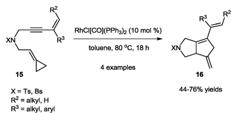
Scheme 20 Rhodium(i)-catalyzed [3 + 2] intramolecular cycloaddition of alkydenecyclopropane-enyne.
