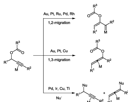
Scheme 2 Transition metal-catalyzed reactions of propargylic esters.
