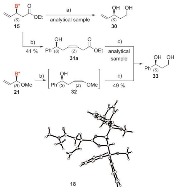
Scheme 8. Assignment of absolute configuration. a) LiAlH 4 , THF, −78 °C → RT, 2 h, then H 2 O 2 , 2 h; b) PhCHO, CH 2 Cl 2 , 0 °C → RT; c) i) O 3 , CH 2 Cl 2 , −78 °C, then Me 2 S; ii) LiAlH 4 , THF 0 °C, 1 h.
