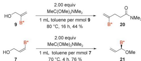
Scheme 6. Rearrangements using Eschenmoser conditions. [24]
