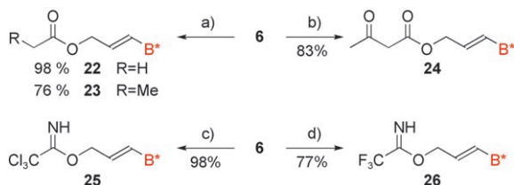
Scheme 7. a) Et 3 N, cat. DMAP, CH 2 Cl 2 , Ac 2 O for 22 or (EtCO) 2 O for 23 ; b) THF, DMAP, diketene, RT, 23 h; c) 0.20 equiv NaH, Et 2 O, 0 °C, 1.20 equiv Cl 3 CCN; d) 6.60 equiv F 3 CCONH 2 , 19.2 equiv DMSO, CH 2 Cl 2 , -78 °C, 6.00 equiv (COCl) 2 , 18.0 equiv Et 3 N, 2.00 equiv DBU, then 1.00 equiv 6 .
