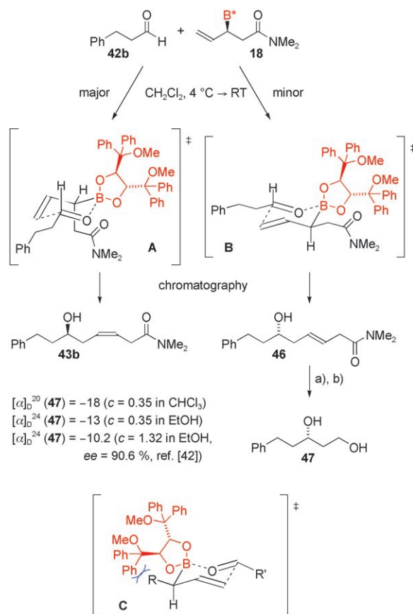
Scheme 11. a) \text{O}_3 , \text{CH}_2\text{Cl}_2 , -78^\circ\text{C} ; \text{Me}_2\text{S} . b) \text{LiAlH}_4 , THF, 56 % over 2 steps.
