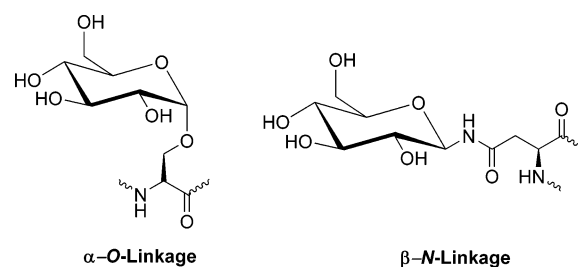
FIGURE 1. \alpha -O-Glycosidic and \beta -N-glycosidic linkages between carbohydrate and peptides.
