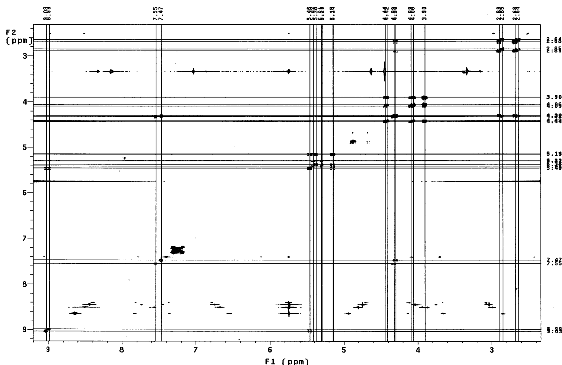
FIGURE 4. ^1\text{H} – ^1\text{H} COSY experiment of 3b in \text{CDCl}_3 at 20 °C.
