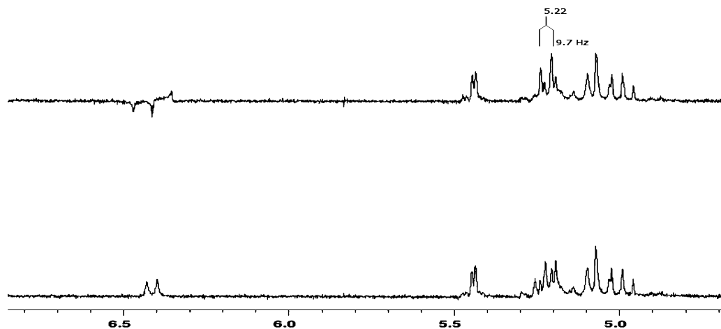
FIGURE 3. Selective decoupling experiment for 3b in \text{CDCl}_3 at 20 °C.
