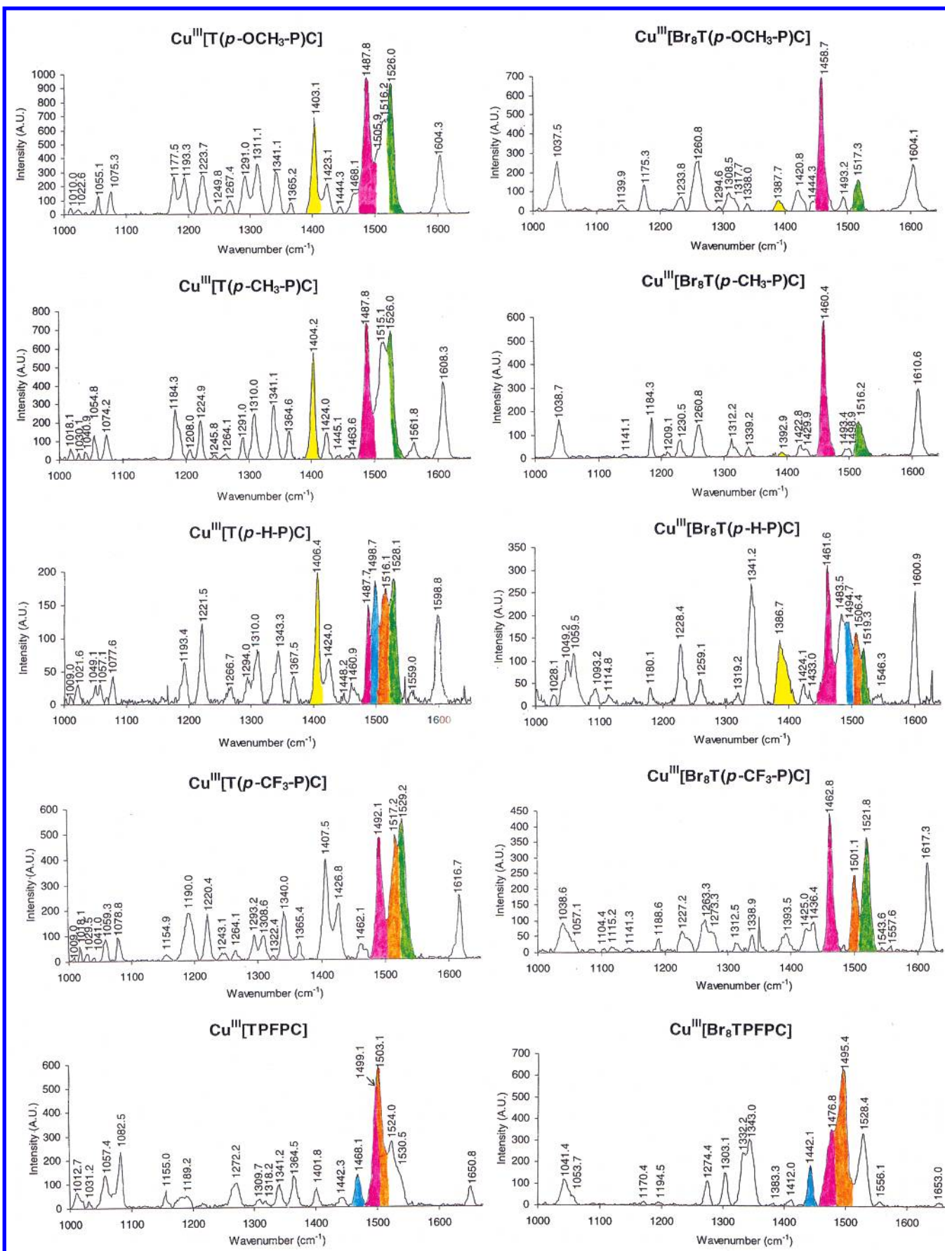
Figure 3. Resonance Raman spectra of Cu(III) triarylcorroles, with the marker bands indicated in color. The spectrum marked [\text{Cu}(\text{Br}_8\text{TPFPC})] may actually be that of [\text{Cu}(\text{Br}_8\text{TPFPC})]^- . See experimental section for additional details.
