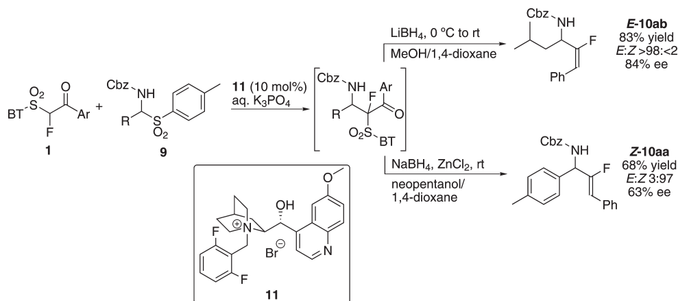
Figure 8. Employment of nucleophiles 1 in the asymmetric organocatalytic formation of dipeptide analogues 10. Reactions performed as in Table 4 at –30 °C with catalyst 11 (10 mol %) instead of TBAB. See Supporting Information for further details.
