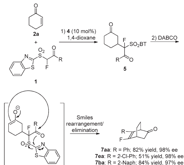
Figure 4. Formation of monofluorinated bicyclo[2.2.2]oct-5-en-2-ones (see Supporting Information for detailed reaction conditions).
