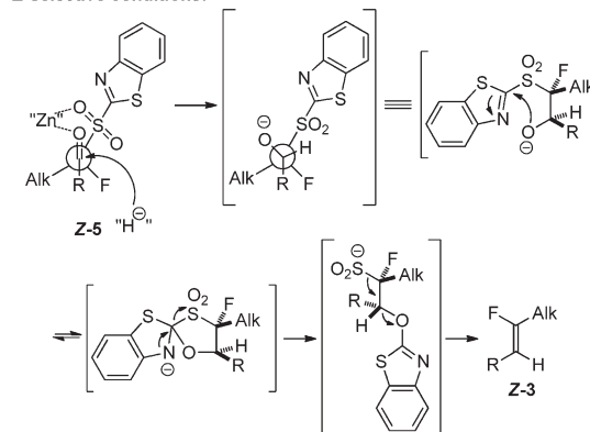
Figure 5. Mechanistic rationale for the observed E : Z -selectivities.
